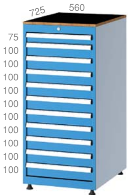
57201 725 X 560 X 1230 mm 11 Adet / Pieces
