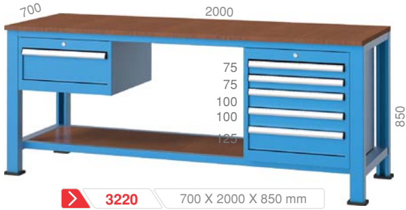
3220 700 X 2000 X 850 mm 6 Adet / Pieces
