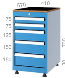
1071 570 X 410 X 730 mm 5 Adet / Pieces
