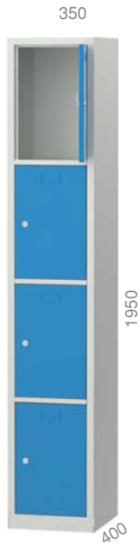
➤ 6062 400 X 350 X 1950 mm
