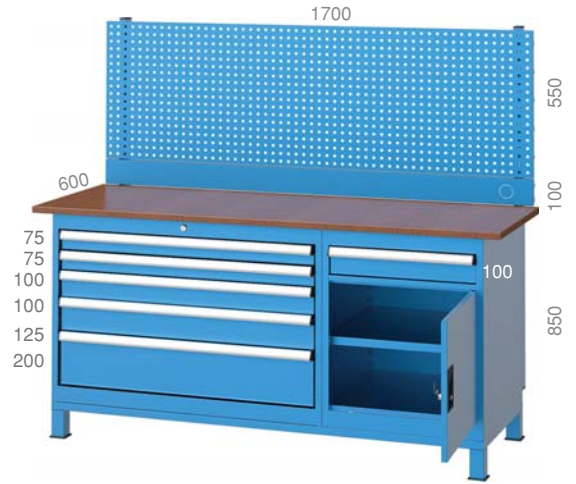
3485 600 X 1700 X 1500 mm
