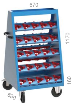
2300 670 X 630 X 1330 mm 50 Adet / Pieces
