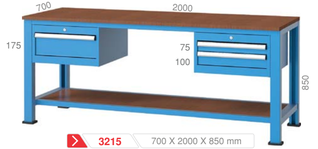
3215 700 X 2000 X 850 mm 3 Adet / Pieces
