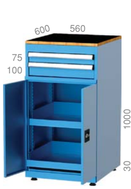
5110 600 X 560 X 1030 mm 2 Adet / Pieces
