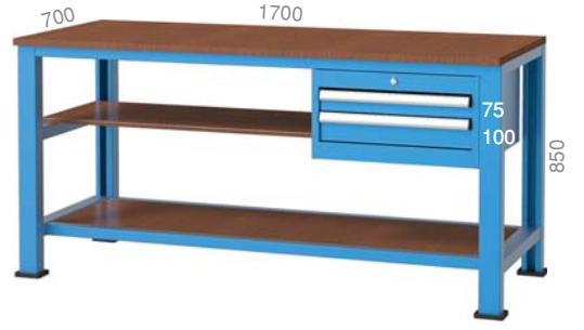
3705 700 X 1700 X 850 mm
