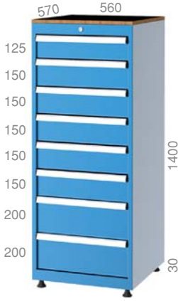
5402 570 X 560 X 1430 mm 8 Adet / Pieces
