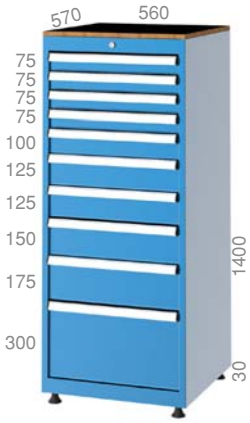
5400 570 X 560 X 1430 mm 10 Adet / Pieces
