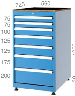
57100 725 X 560 X 1030 mm 7 Adet / Pieces
