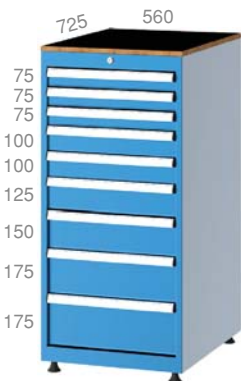
57200 725 X 560 X 1230 mm 9 Adet / Pieces
