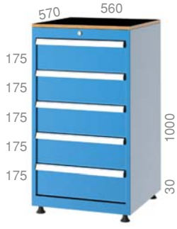
5102 570 X 560 X 1030 mm 5 Adet / Pieces
