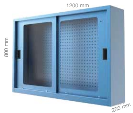
3050 250 X 1200 X 800 mm
