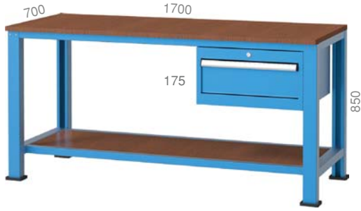
3745 700 X 1700 X 850 mm
