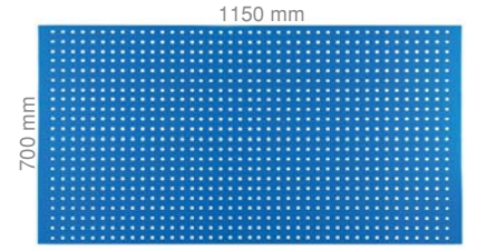
3010 700 X 1150 X 20 mm AS-1107
