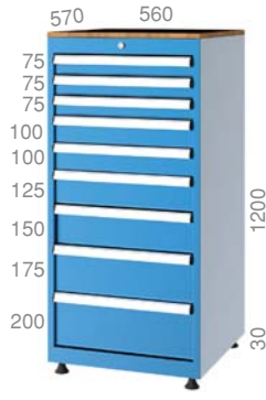
5200 570 X 560 X 1230 mm 9 Adet / Pieces
