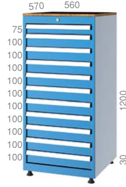
5201 570 X 560 X 1230 mm 11 Adet / Pieces
