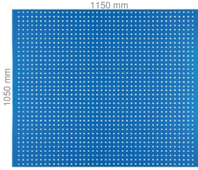
3005 1050 X 1150 X 20 mm AS-1110
