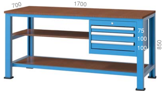
3730 700 X 1700 X 850 mm
