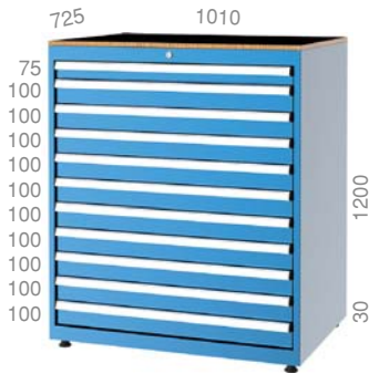
11200 725 X 1010 X 1230 mm 11 Adet / Pieces
