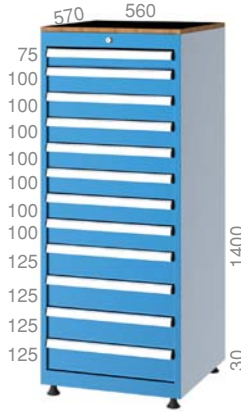
5401 570 X 560 X 1430 mm 12 Adet / Pieces
