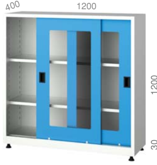
6555 400 X 1200 X 1230 mm
