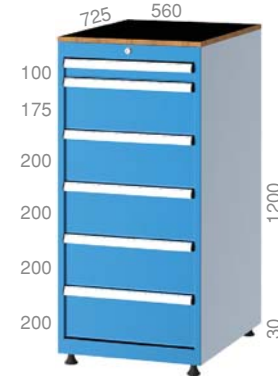
57202 725 X 560 X 1230 mm 6 Adet / Pieces
